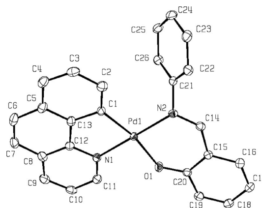
Figure 5. ORTEP diagram of II4 . Thermal ellipsoids are drawn at the 50% probability level.
