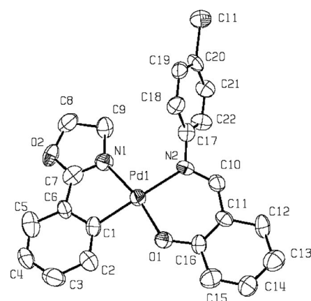
Figure 8. X-ray crystal structure of III5 . Thermal ellipsoids are drawn at the 50% probability. Hydrogens are omitted for clarity.
