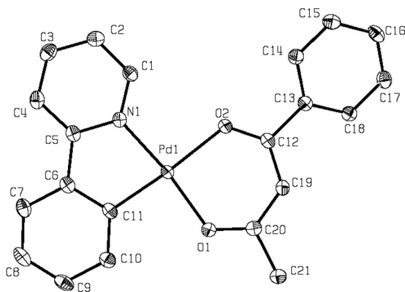
Figure 2. X-ray crystal structure of I3 . Thermal ellipsoids are drawn at the 50% probability. Hydrogen atoms are omitted for clarity.
