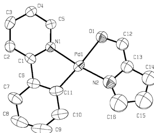
Figure 3. An ORTEP representation of I6 . Thermal ellipsoids are drawn at the 50% probability.
