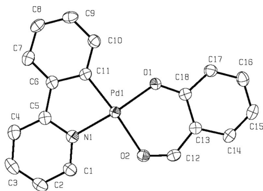
Figure 1. ORTEP diagram of complex II with the atom numbering scheme. Thermal ellipsoids are drawn at the 50% probability level.
