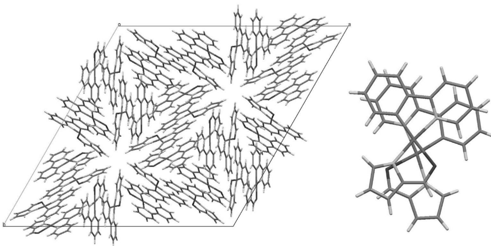
Figure 4. Molecular packing diagram of complex 16 and perspective view of the alignment of the two molecules.
