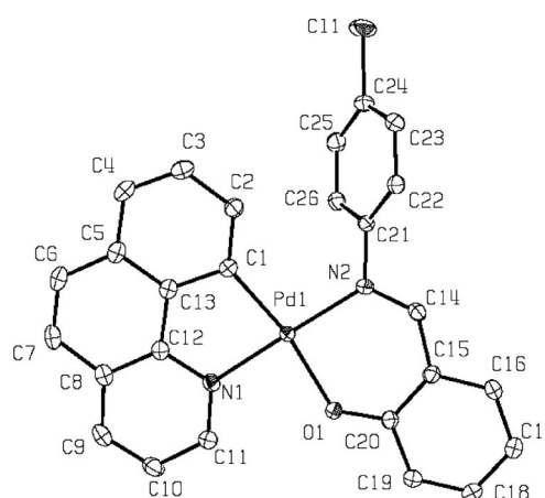
Figure 6. Molecular structure of II5 with the labelling scheme. Thermal ellipsoids are drawn at the 50% probability level. Hydrogen atoms have been omitted for clarity.
