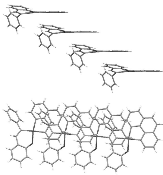
Figure 7. Packing diagram in II4 .
